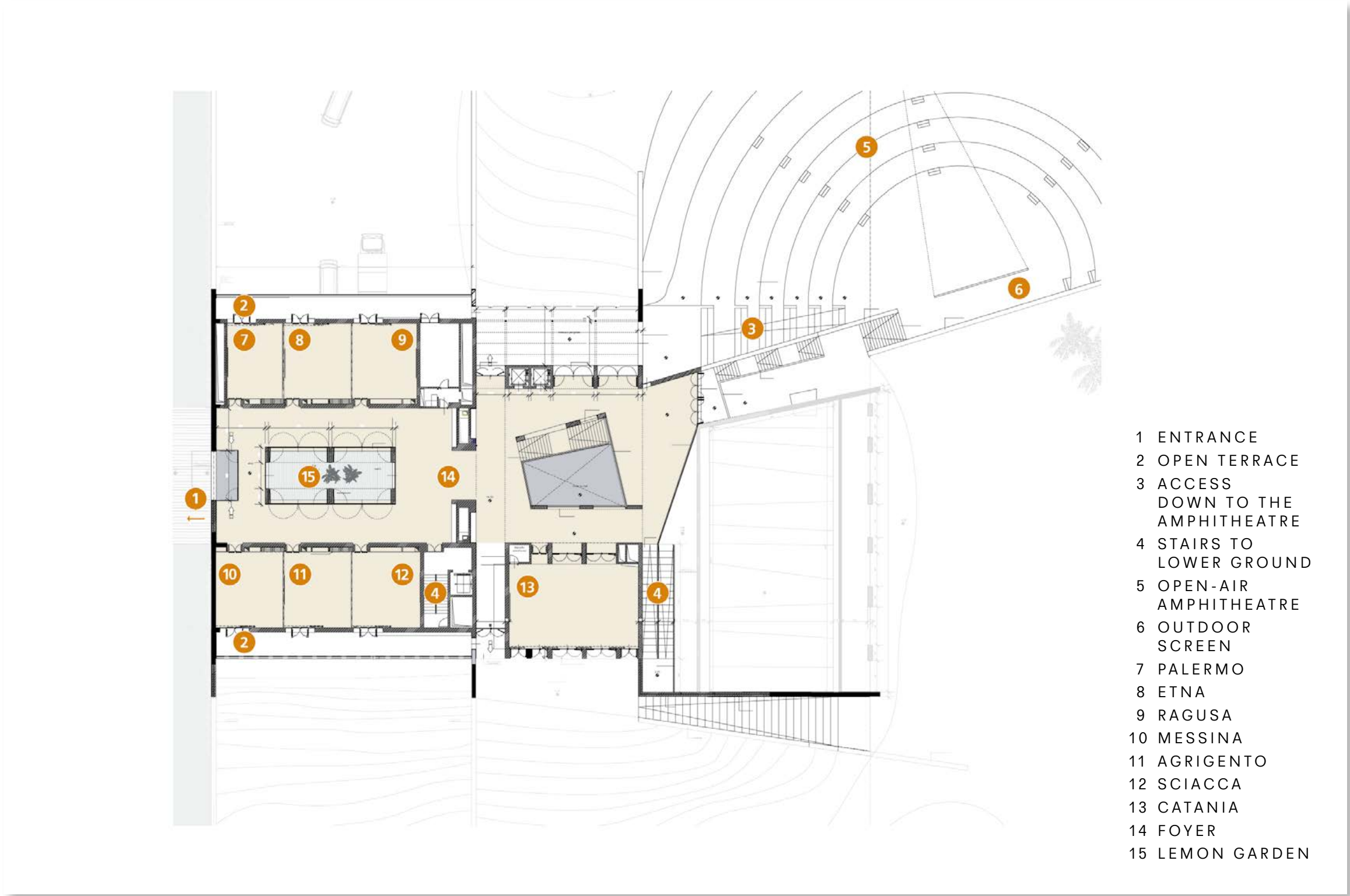
FLOORPLAN – GROUND FLOOR
